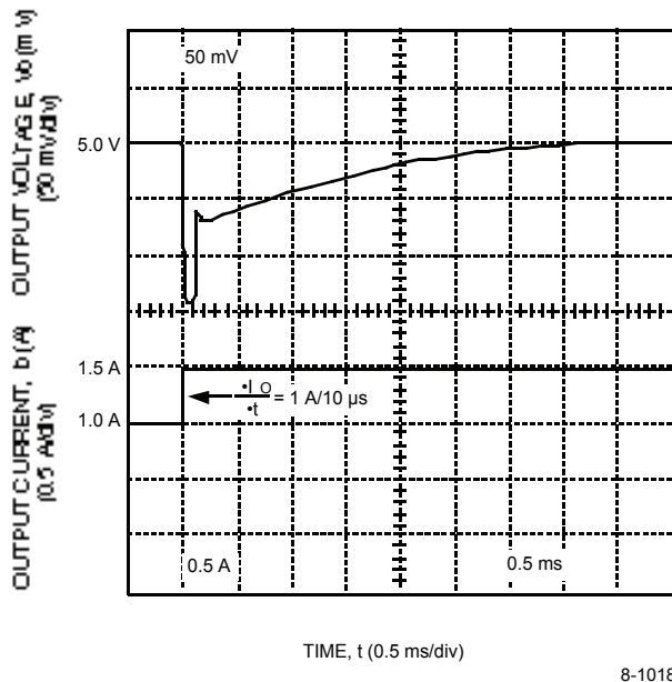
Figure 7. CC025 Dual-Output-Series Typical 5 V Output Voltage Response to a Step Load Change from 50% to 75% of I_{o, max} at V_i = V_{i, nom} and T_c = 25\text{ }^\circ\text{C}
