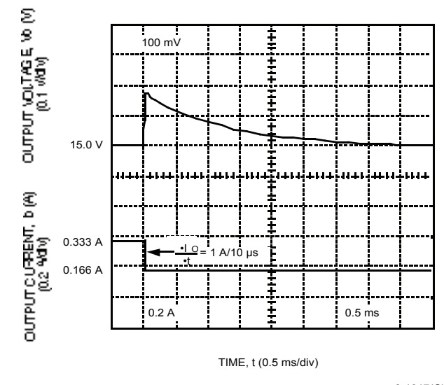
Figure 6. CC025 Dual-Output-Series Typical 15 V Output Voltage Response to a Step Load Change from 50% to 25% of I_{o, max} at V_i = V_{i, nom} and T_c = 25\text{ }^\circ\text{C}
