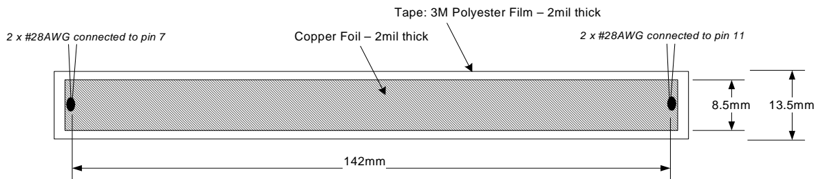
Figure 5 – Transformer Build Diagram.
