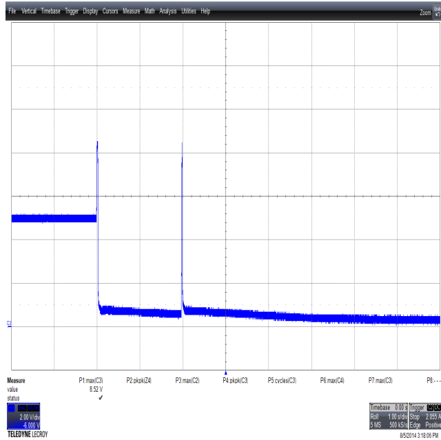
Figure 26 – 5 V Output in Response to Open Loop R5 = 20 \text{ }\Omega to Configure Latching Shutdown. Output Voltage 2 V / div., 1 s / div.
