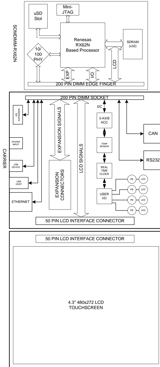
Figure 4 – DK-TS-KIT System Block Diagram
