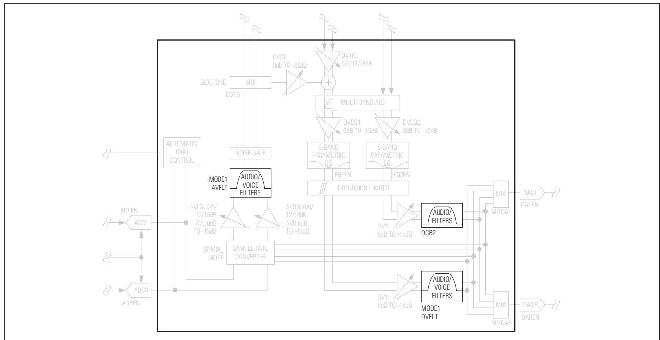
Figure 19. Digital Passband Filtering Block Diagram
