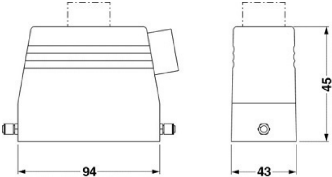
Dimensioned drawing
